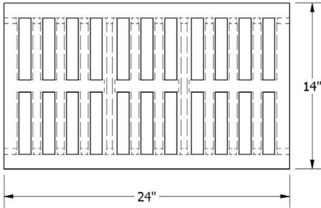
GRATES H-20 Rated, 65 LBS
