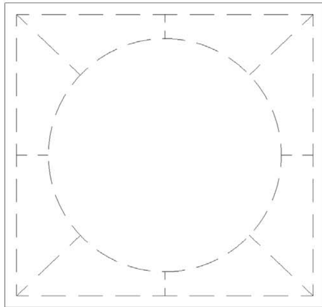
#6 REBAR STEEL REINFORCEMENT DETAIL
